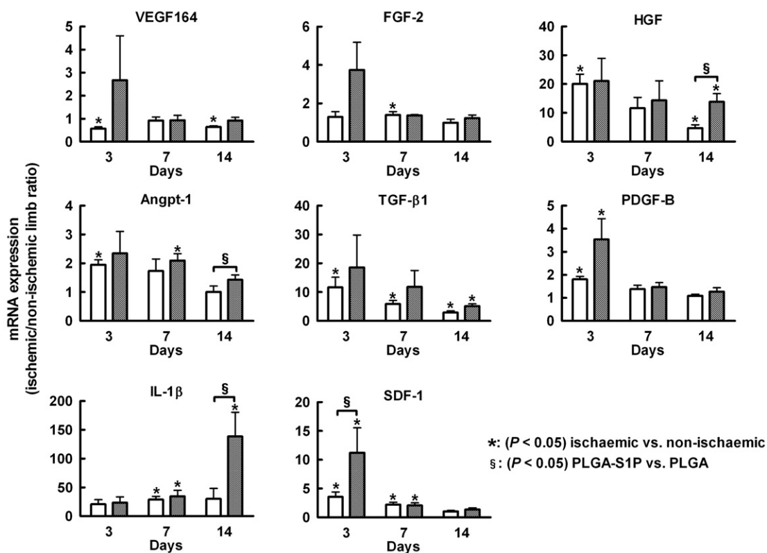
Fig. 5. mRNA expression of angiogenic factors in ischemic hindlimb muscle in C57BL/6 mice. mRNA expression levels of angiogenic factors in calf muscle from PLGA-S1P treated (stippled) and PLGA treated (open) mice on postoperative days 3, 7, and 14 were determined by real-time PCR. GAPDH was used as an endogenous control. Data are expressed as the ratio of the values in ischemic over non-ischemic muscle and represent the mean ± S.E.M. ( n = 5 or 6 mice per group). * P < 0.05 , ischemic limb versus non-ischemic limb; § P < 0.05 , the PLGA-S1P treated mice versus the PLGA treated mice.
