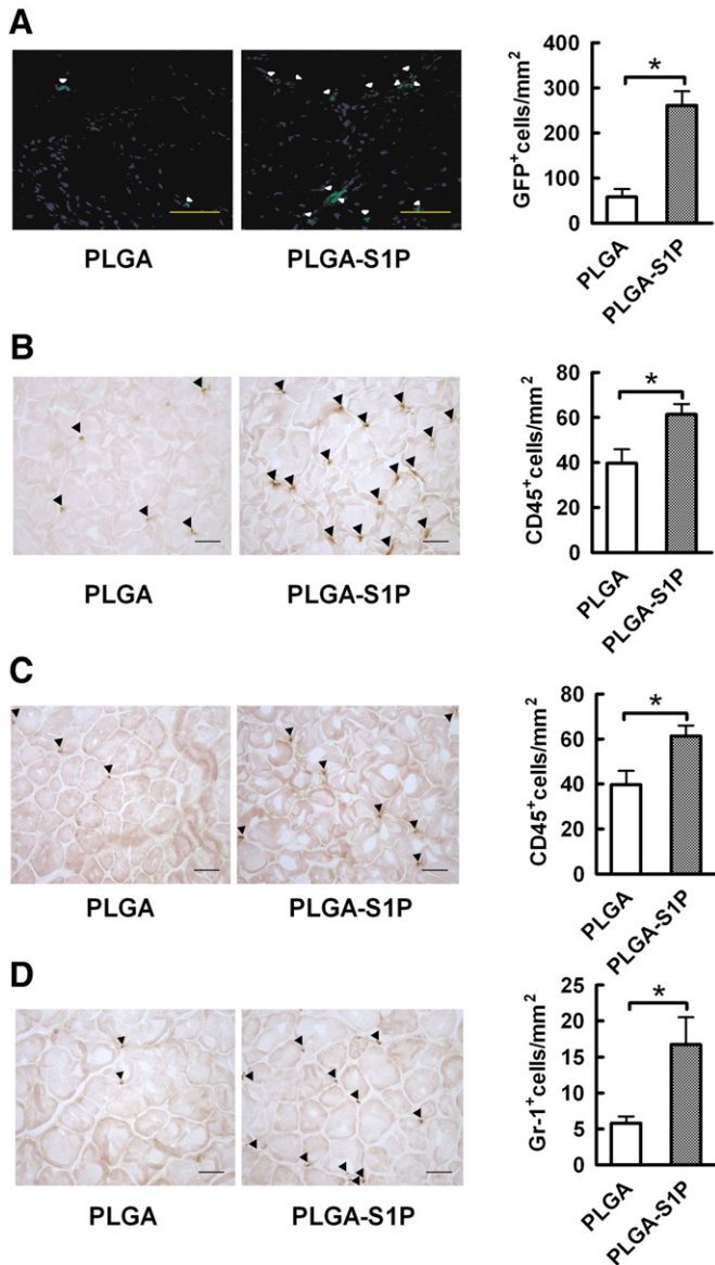
Fig. 8. PLGA-S1P promotes bone marrow-derived cells (BMDCs) recruitment into the ischemic area in C57BL/6 mice. (A) GFP-positive cell recruitment into the ischemic area is promoted by PLGA-S1P. Ischemic calf muscle was excised on postoperative day 28 from C57BL/6 mice that had received transplantation of bone marrow (BM) cells from GFP-transgenic mice 4 weeks before the operation, and GFP-positive BMDCs in muscle were counted. B, C, and D, CD11b- (B), CD45- (C), or Gr-1- (D) positive cells recruitment into the ischemic area are promoted by PLGA-S1P. Sections of the calf muscle in PLGA treated and PLGA-S1P treated mice were probed with anti-CD11, anti-CD45, or anti-Gr-1 immunostaining, and CD11b-, CD45-, or Gr-1-positive cells were counted. Quantitative analyses of positive cell number are also shown. Data represent the mean \pm S.E.M. ( n = 6 mice per group). * P < 0.05 , the PLGA-S1P treated mice versus the PLGA treated mice. Scale bar = 50 \mu m.
