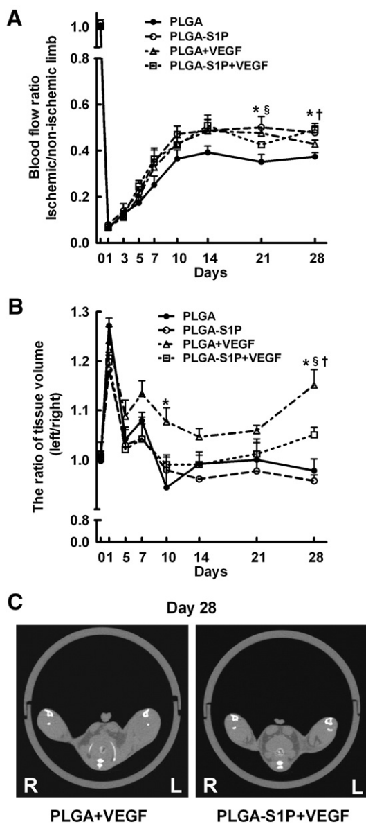
Fig. 3. Effects of either alone of PLGA-S1P and VEGF and the combination on blood flow recovery (A) and tissue edema (B, C) in C57BL/6 mice. Ischaemic/non-ischaemic limb LDBF ratio value (A) and ischaemic/non-ischaemic tissue volume evaluated by X-ray imaging analysis (B) in mice that received either PLGA-S1P (180 pmol total S1P) or PLGA alone at 3-day interval with or without daily injections of 56 ng VEGF for 28 days. Data represent the mean \pm S.E.M. ( n = 8 mice per group). In A: * P < 0.05 , PLGA treated mice versus PLGA-S1P treated mice; ^{\S}P < 0.05 , PLGA treated mice versus PLGA plus VEGF treated mice; ^{\dagger}P < 0.05 , PLGA treated mice versus the PLGA-S1P plus VEGF treated mice. In B, * P < 0.05 , the PLGA treated mice versus the PLGA plus VEGF treated mice. ^{\S}P < 0.05 , the PLGA plus VEGF treated mice versus the PLGA-S1P plus VEGF treated mice; ^{\dagger}P < 0.05 , the PLGA-S1P treated mice versus the PLGA with VEGF treated mice. (C) Representative X-ray images on postoperative day 28 are shown. R: right; L: left.
