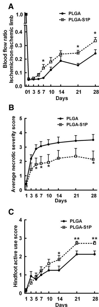
Fig. 2. Local PLGA-S1P injections enhance the blood flow recovery (A), inhibit the tissue damage (B), and improve the functional recovery (C) of the limbs in Balb/c mice. (A) Ischaemic/non-ischaemic limb LDBF ratio value in mice that received either PLGA-S1P (180 pmol total S1P) or PLGA alone at 3-day interval for 28 days. (B) Mean severity scores for tissue necrosis. The severity of hind limb tissue necrosis was serially assessed after operation. (C) Spontaneous active use scores of left hindlimbs. The functional recovery of hind limb was serially assessed after operation. Data represent the mean \pm S.E.M. ( n = 15 mice per group). * P < 0.05 and ** P < 0.01 versus the PLGA treated mice.
