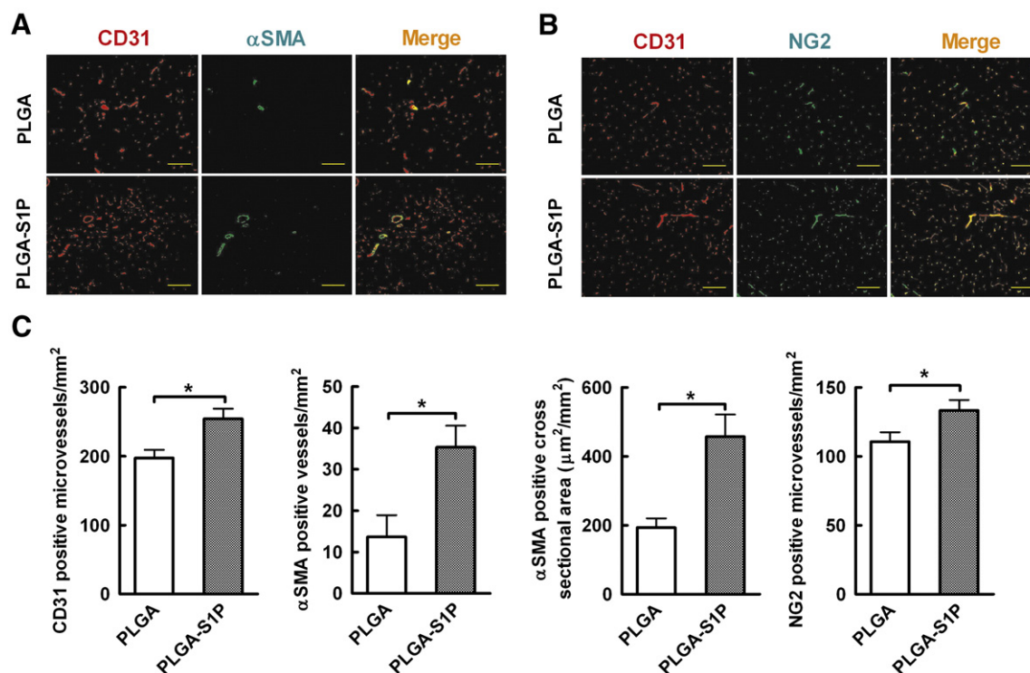
Fig. 4. PLGA-S1P stimulates angiogenesis and arteriogenesis in C57BL/6 mice. A and B, EC marker CD31 (red) and smooth muscle cell marker αSMA (A) and pericyte marker (B) were detected by double immunofluorescence (green) in the ischemic hindlimb of PLGA treated (upper panel) and PLGA-S1P treated (lower panel) mice. Representative immunofluorescence images of either marker and merge images are shown. (C) CD31 positive microvessels, αSMA positive vessels, αSMA positive vascular area and NG2 positive microvessels were quantified by Image J software (NIH). Data represent the mean ± S.E.M. ( n = 4 or 5 mice per group). * P < 0.05 and ** P < 0.01 versus the PLGA treated mice. Scale bar = 100 μm.
