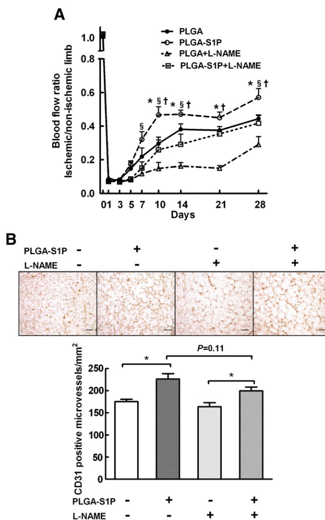
Fig. 7. Effect of N \omega -nitro-L-arginine methylester (L-NAME) on PLGA-S1P induced stimulation of blood flow recovery in C57BL/6 mice. (A) Ischaemic/non-ischaemic limb LDBF ratio value in mice of the 4 experimental groups; PLGA treated mice with or without L-NAME, PLGA-S1P treated mice with or without L-NAME. Data represent the mean \pm S.E.M. ( n = 8 mice per group). * P < 0.05 , PLGA-S1P treated mice versus PLGA treated mice; § P < 0.05 , PLGA-S1P treated mice versus PLGA-S1P with L-NAME treated mice; † P < 0.05 , PLGA treated mice versus PLGA with L-NAME treated mice. (B) Immunohistochemical analysis of CD31 in ischemic hindlimbs of PLGA treated and PLGA-S1P treated mice with or without L-NAME. Shown are representative images (upper panel) from calf muscle on postoperative day 28. Quantitative analysis of CD31-positive microvessel density is also shown (lower panel). Data represent the mean \pm S.E.M. ( n = 5 mice per group). * P < 0.05 . Scale bar = 100 \mu\text{m} .
