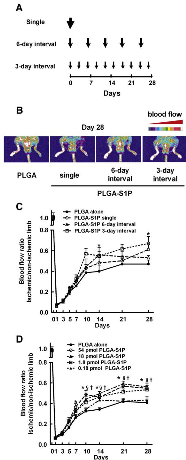
Fig. 1. Local PLGA-S1P injections enhance the blood flow recovery in C57BL/6 mice. (A) Protocol of administration of PLGA-S1P microparticles. (B) Laser Doppler blood flow (LDBF) pseudocolour images, as determined with an LDBF analyser, in mice that received either PLGA-S1P (180 pmol total S1P) at single bolus, 6-day interval or 3-day interval or PLGA alone at 3-day interval on postoperative day 28. (C) Ischaemic/non-ischaemic limb LDBF ratio value in mice that received either PLGA-S1P (180 pmol total S1P) at various administration interval or PLGA alone at 3-day interval for 28 days. Data represent the mean \pm S.E.M. ( n = 8 mice per group). * P < 0.05 , PLGA-S1P at 3-day interval versus the PLGA. (D) Ischaemic/non-ischaemic limb LDBF ratio value in mice that received either various doses of PLGA-S1P or PLGA alone at 3-day interval for 28 days. Data represent the mean \pm S.E.M. ( n = 8 mice per group). * P < 0.05 , the 54 pmol PLGA-S1P treated mice versus the PLGA treated mice; † P < 0.05 , the 18 pmol PLGA-S1P treated mice versus the PLGA treated mice; ‡ P < 0.05 , the 1.8 pmol PLGA-S1P treated mice versus the PLGA treated mice.
