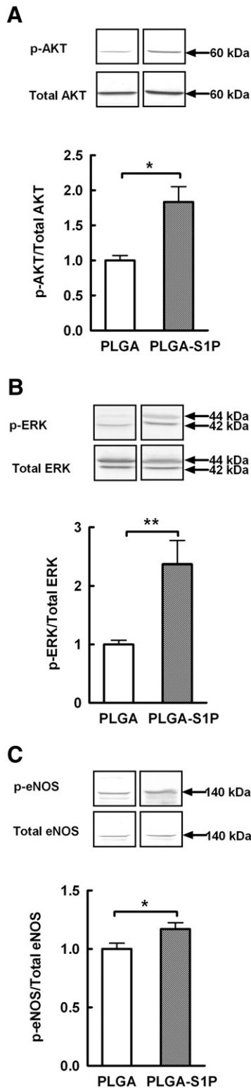
Fig. 6. Phosphorylation of Akt, ERK and eNOS in ischemic muscle following injections of PLGA-S1P or PLGA in C57BL/6 mice. Muscle tissue homogenates from PLGA-S1P treated (filled) and PLGA treated (open) mice on postoperative day 28 were subjected to Western blot using antibodies against phospho-Akt and total Akt (A), phospho-ERK and total ERK (B), and phospho-eNOS and total eNOS (C) as described in "Materials and methods". Quantitative analyses of band densities are also shown. Data represent the mean \pm S.E.M. ( n=5 mice per group). * P<0.05 , ** P<0.01 versus the PLGA treated mice.
